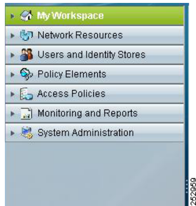
Figure 5-3 Navigation Pane
